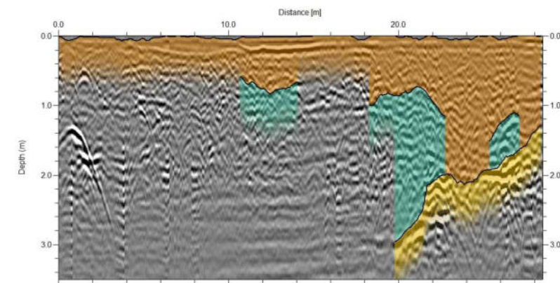
GPR LINE 066
