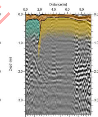
GPR LINE 062
