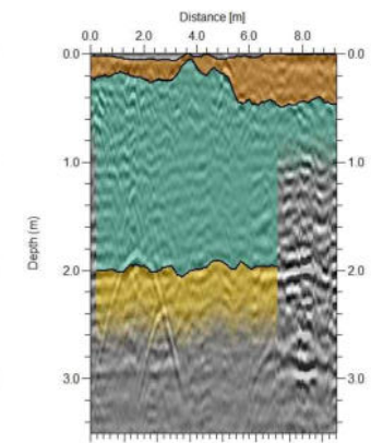
GPR LINE 058
